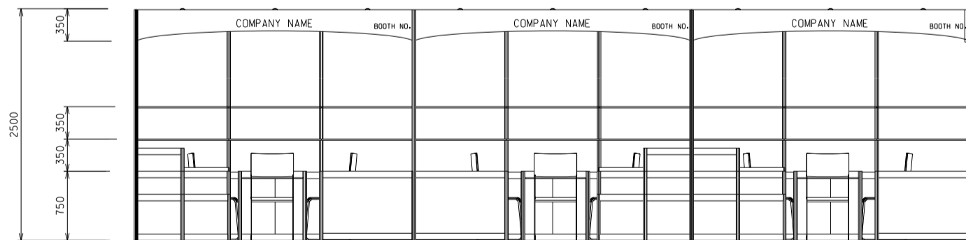
ELEVATION 9M(W) X 3M(D) X 2.5M(H) RIGHT CORNER BOOTH B
